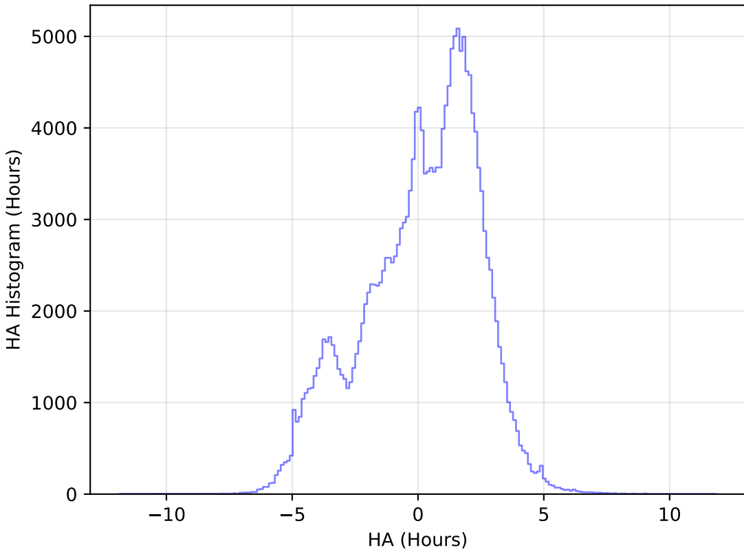
too_elab_r32_d2_ugrizy_v3.4_10yrs All sky g band: HA Histogram
