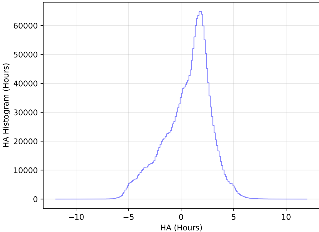
too_elab_r32_d2_ugrizy_v3.4_10yrs All sky all bands: HA Histogram
