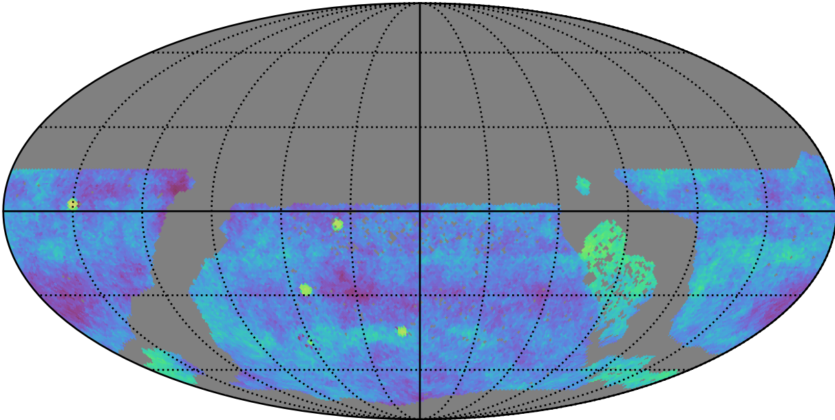
too_elab_r32_d2_ugrizy_v3.4_10yrs gri WFD: Fraction of visits in pairs (20-90 min)
