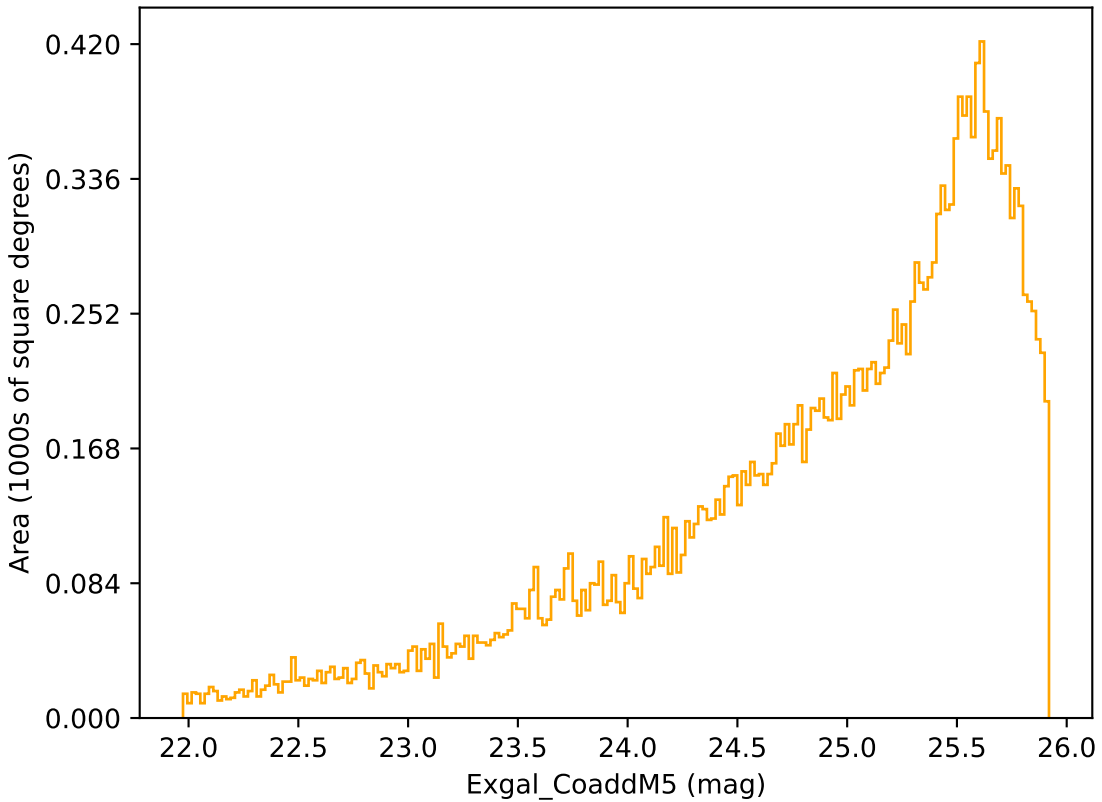
too_elab_r32_d2_ugrizy_v3.4_10yrs Yr 3-4 r band: Exgal_CoaddM5
