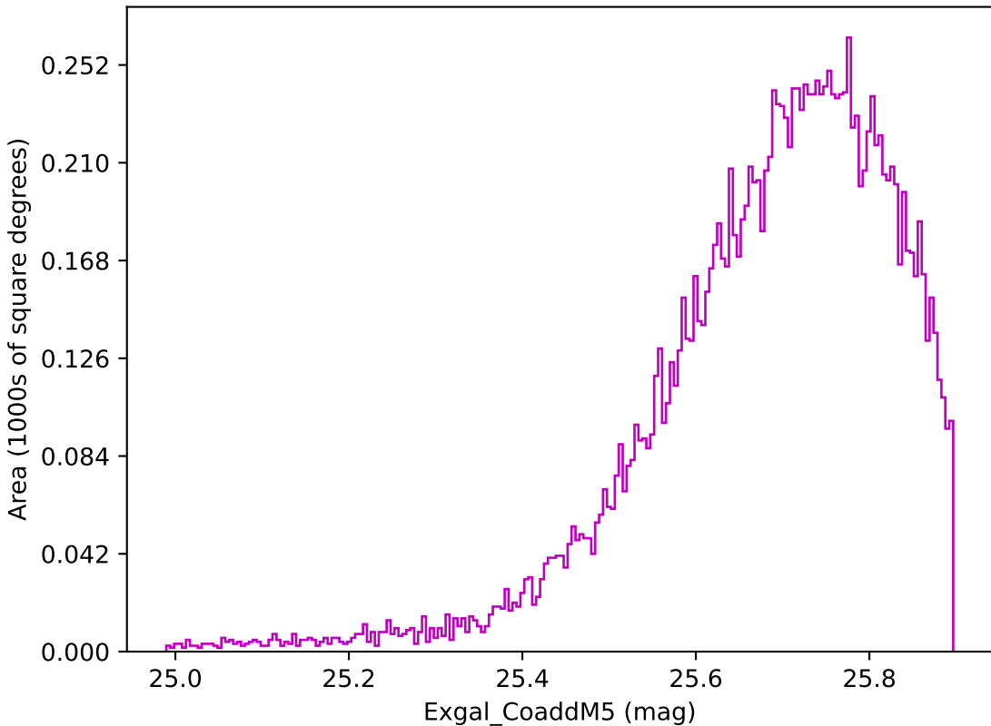
too_elab_r32_d2_ugrizy_v3.4_10yrs WFD z band: Exgal_CoaddM5
