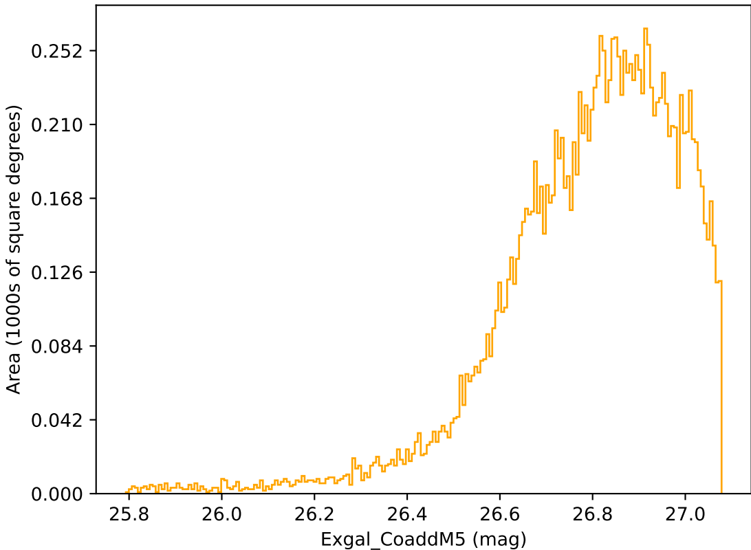
too_elab_r32_d2_ugrizy_v3.4_10yrs WFD r band: Exgal_CoaddM5
