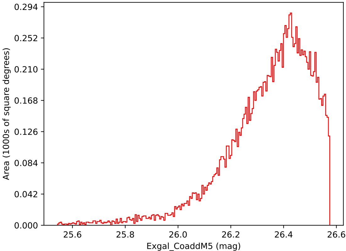
too_elab_r32_d2_ugrizy_v3.4_10yrs WFD i band: Exgal_CoaddM5
