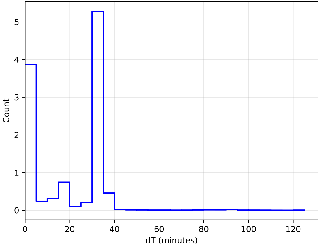
too_elab_r32_d2_ugrizy_v3.4_10yrs WFD: DeltaT Histogram 1e6
