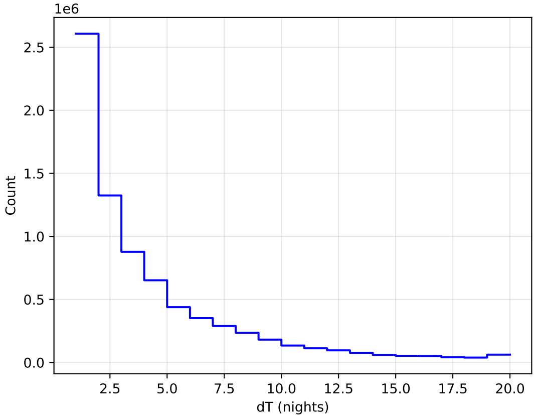
too_elab_r32_d2_ugrizy_v3.4_10yrs WFD all bands: DeltaNight Histogram
