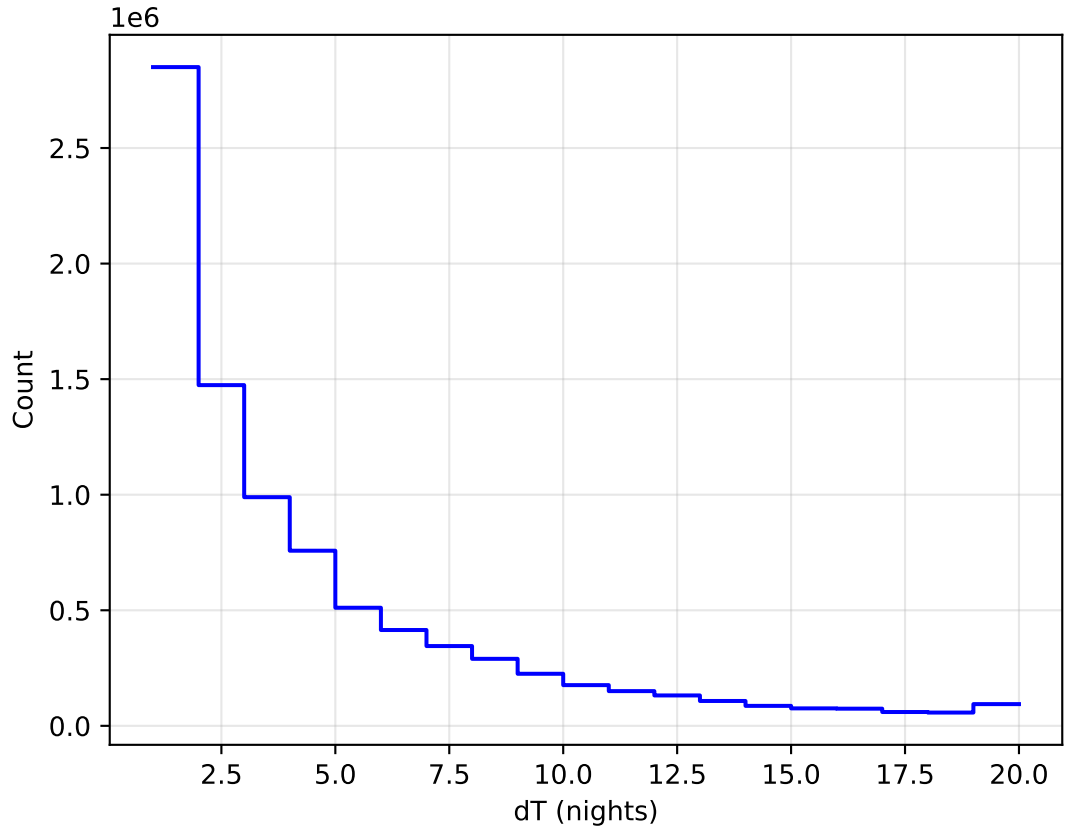
too_elab_r32_d2_ugrizy_v3.4_10yrs All sky all bands: DeltaNight Histogram
