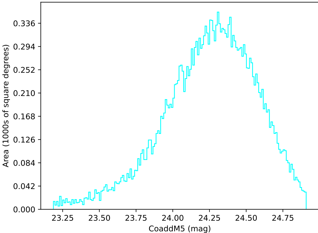
too_elab_r32_d2_ugrizy_v3.4_10yrs Yr 1 u band: CoaddM5
