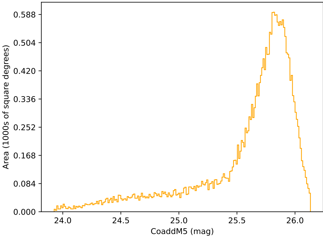
too_elab_r32_d2_ugrizy_v3.4_10yrs Yr 1 r band: CoaddM5
