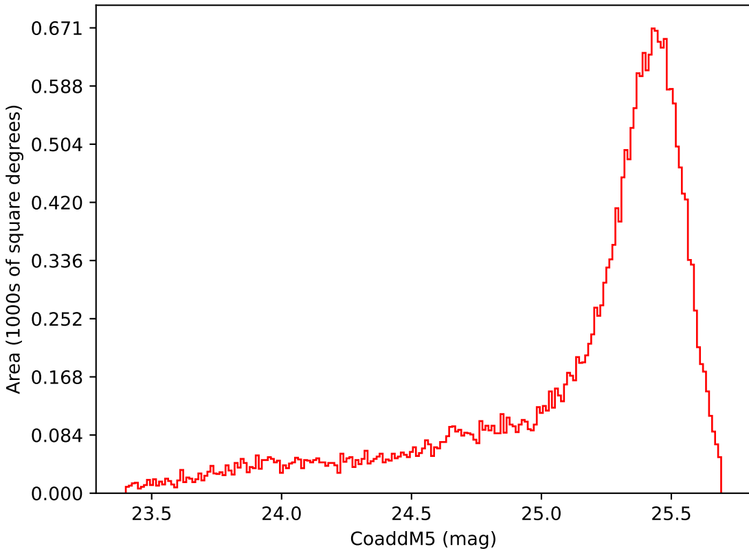
too_elab_r32_d2_ugrizy_v3.4_10yrs Yr 1 i band: CoaddM5
