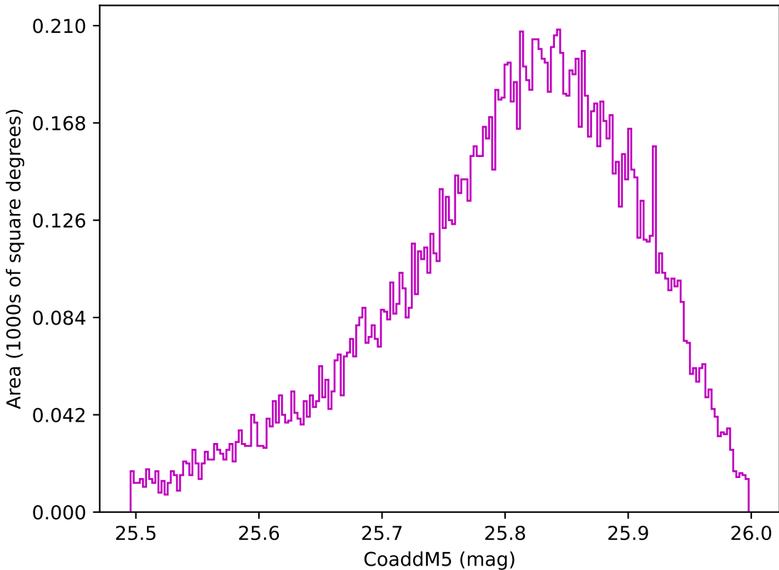
too_elab_r32_d2_ugrizy_v3.4_10yrs WFD z band: CoaddM5
