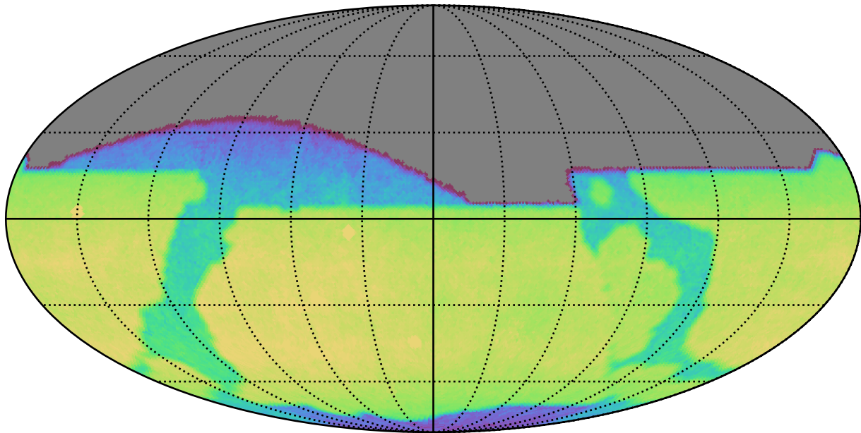
too_elab_r32_d2_ugrizy_v3.4_10yrs All sky z band: CoaddM5
