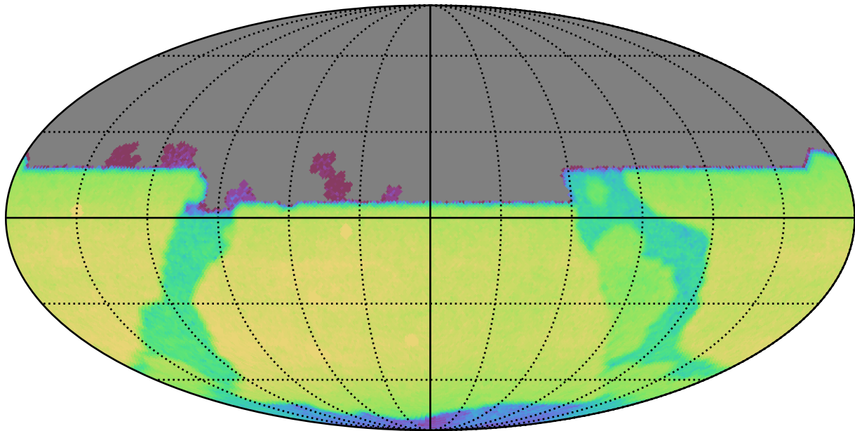
too_elab_r32_d2_ugrizy_v3.4_10yrs All sky y band: CoaddM5
