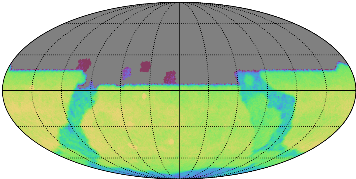
too_elab_r32_d2_ugrizy_v3.4_10yrs All sky u band: CoaddM5
