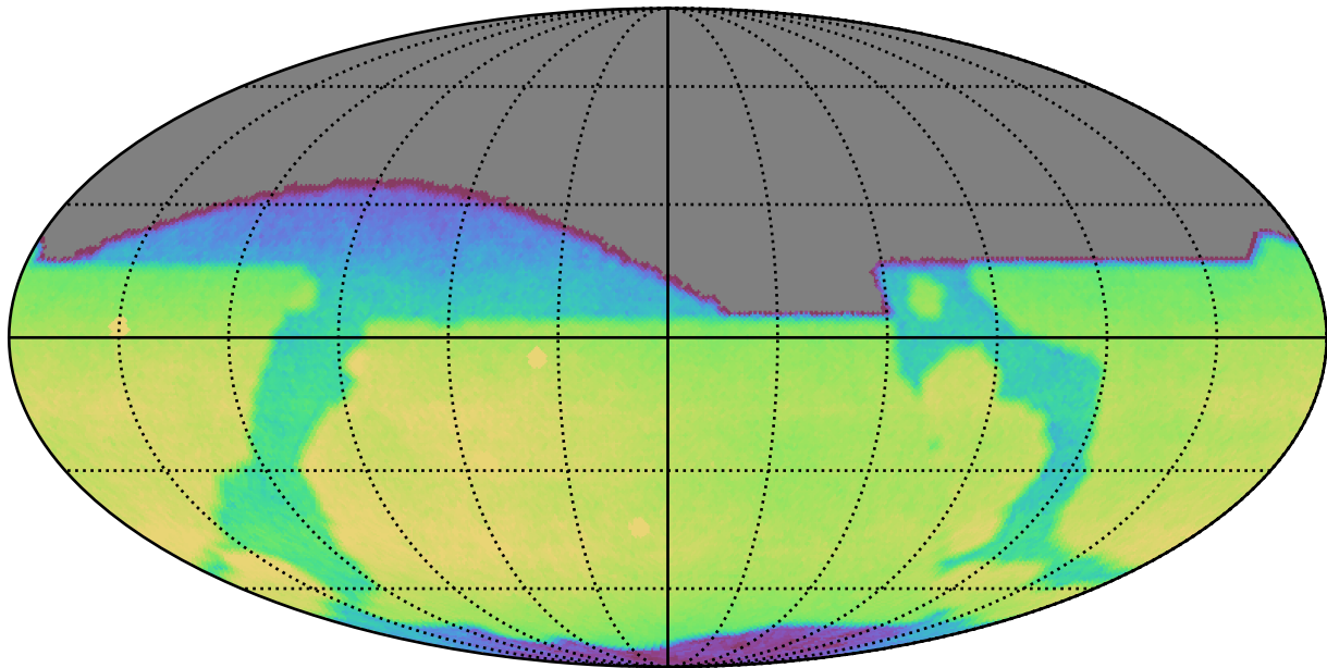
too_elab_r32_d2_ugrizy_v3.4_10yrs All sky r band: CoaddM5
