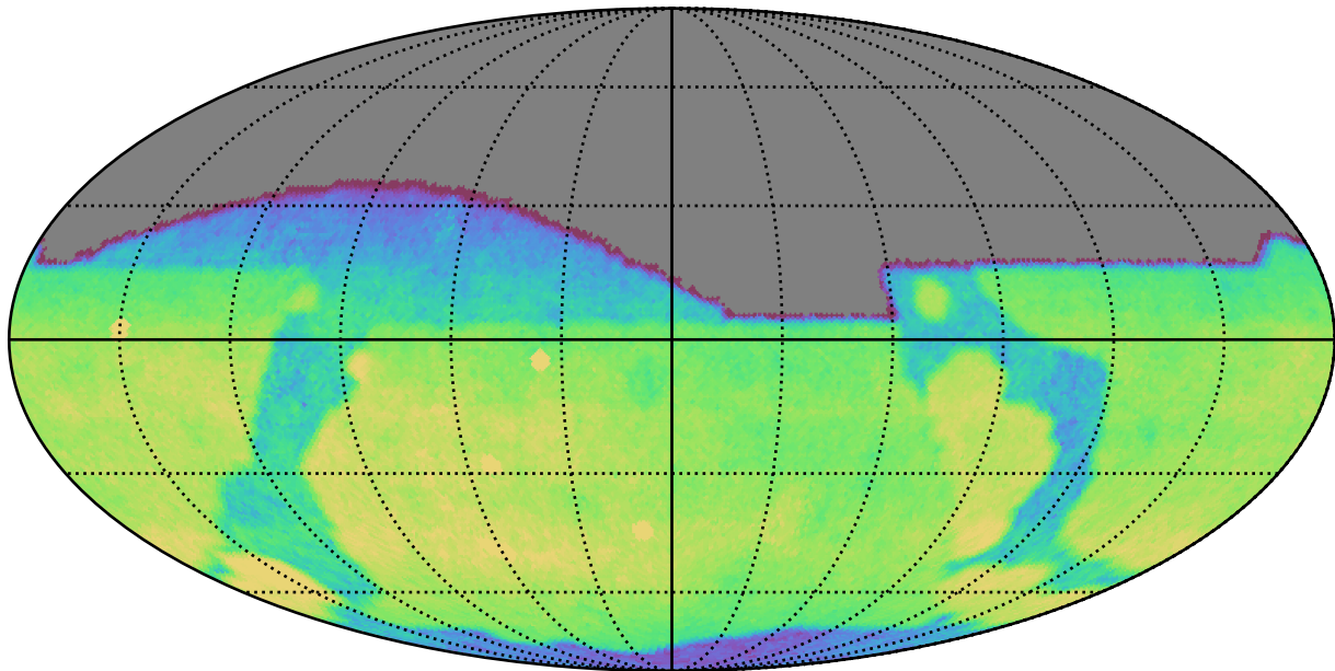
too_elab_r32_d2_ugrizy_v3.4_10yrs All sky g band: CoaddM5
