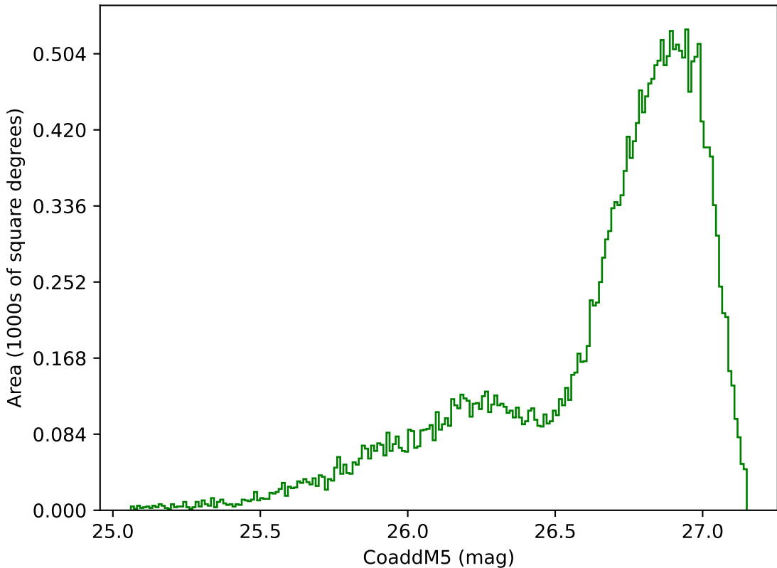
too_elab_r32_d2_ugrizy_v3.4_10yrs All sky g band: CoaddM5
