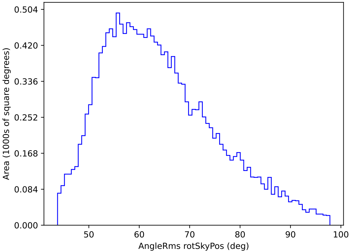
too_elab_r32_d2_ugrizy_v3.4_10yrs WFD u band: AngleRms rotSkyPos
