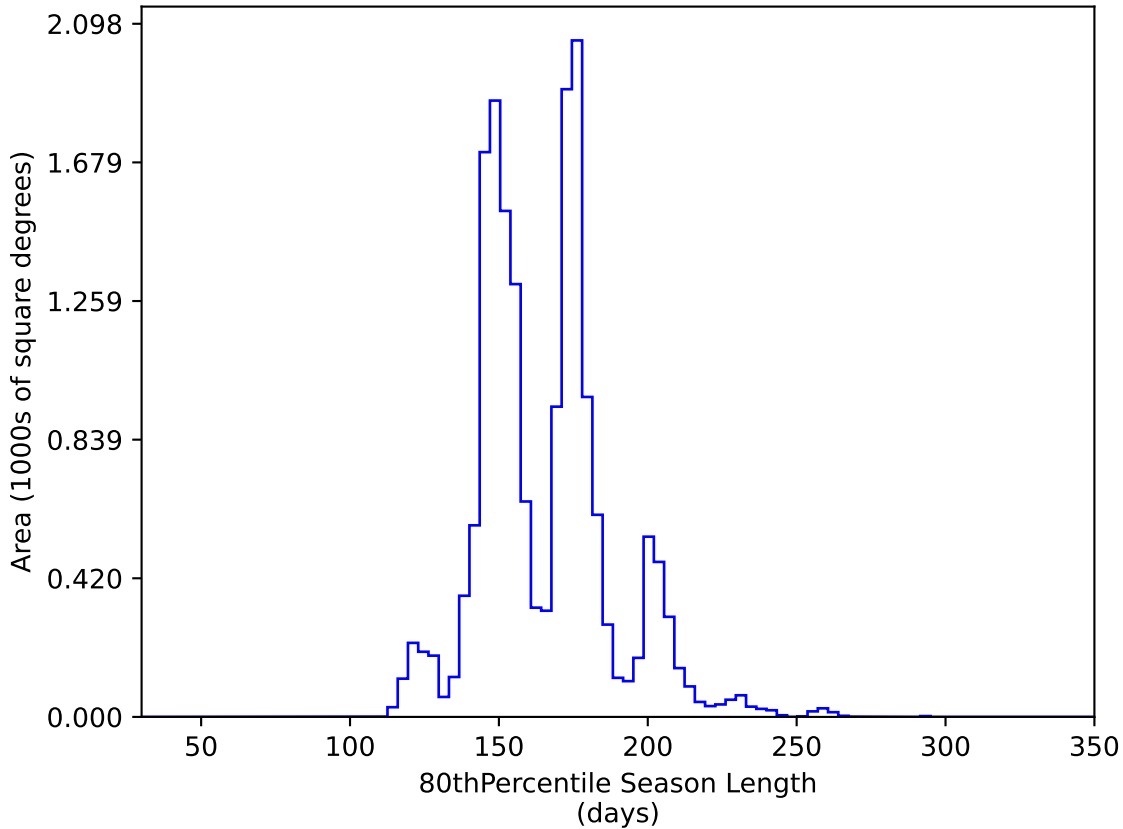
too_elab_r32_d2_ugrizy_v3.4_10yrs WFD y band: 80thPercentile Season Length
