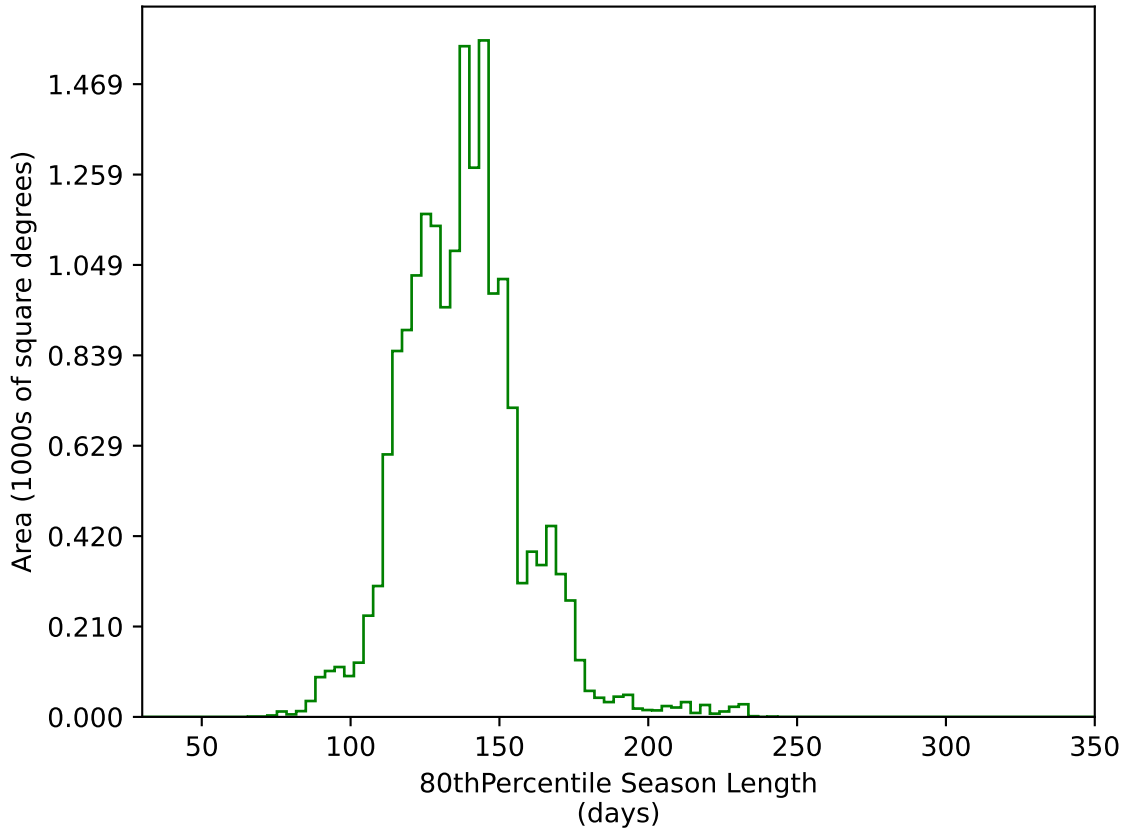
too_elab_r32_d2_ugrizy_v3.4_10yrs WFD g band: 80thPercentile Season Length
