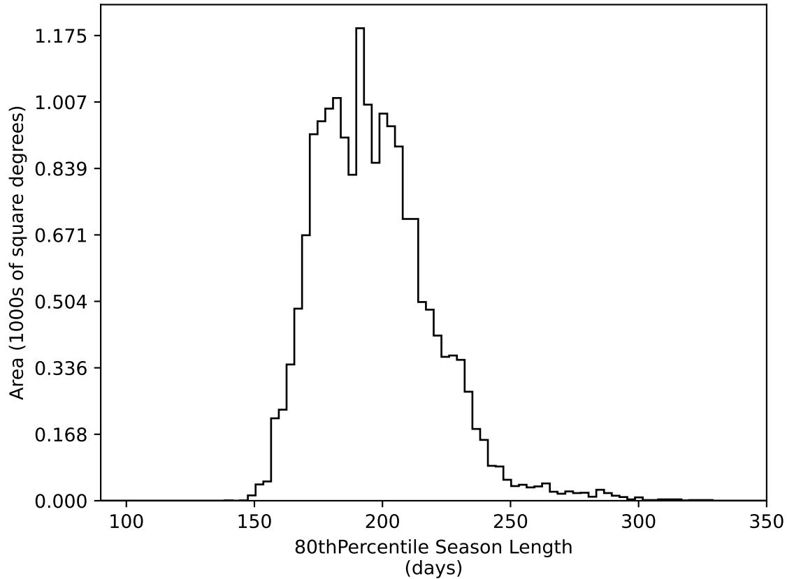
too_elab_r32_d2_ugrizy_v3.4_10yrs WFD all bands: 80thPercentile Season Length
