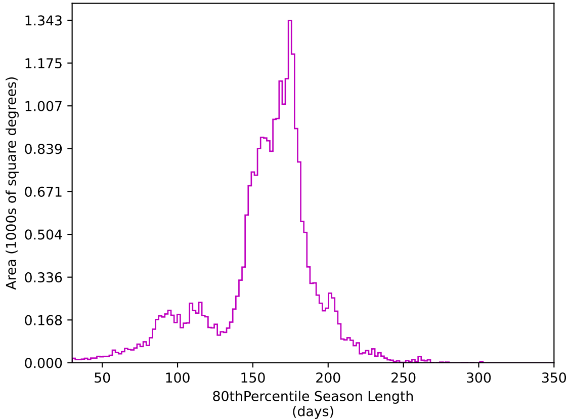
too_elab_r32_d2_ugrizy_v3.4_10yrs All sky z band: 80thPercentile Season Length
