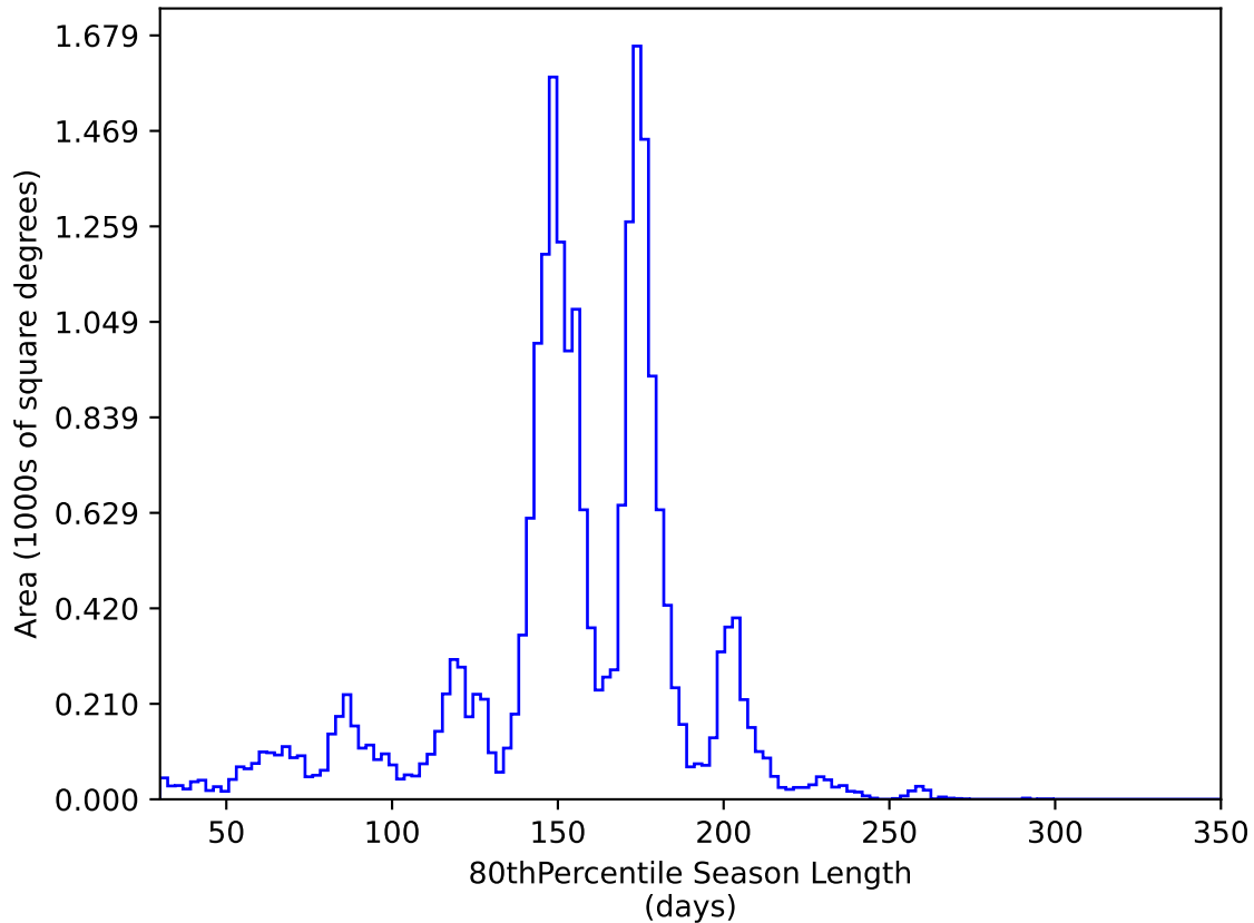
too_elab_r32_d2_ugrizy_v3.4_10yrs All sky y band: 80thPercentile Season Length
