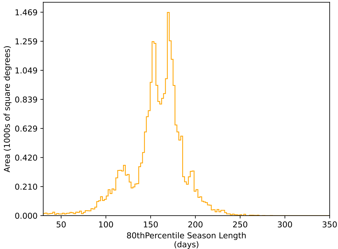
too_elab_r32_d2_ugrizy_v3.4_10yrs All sky r band: 80thPercentile Season Length
