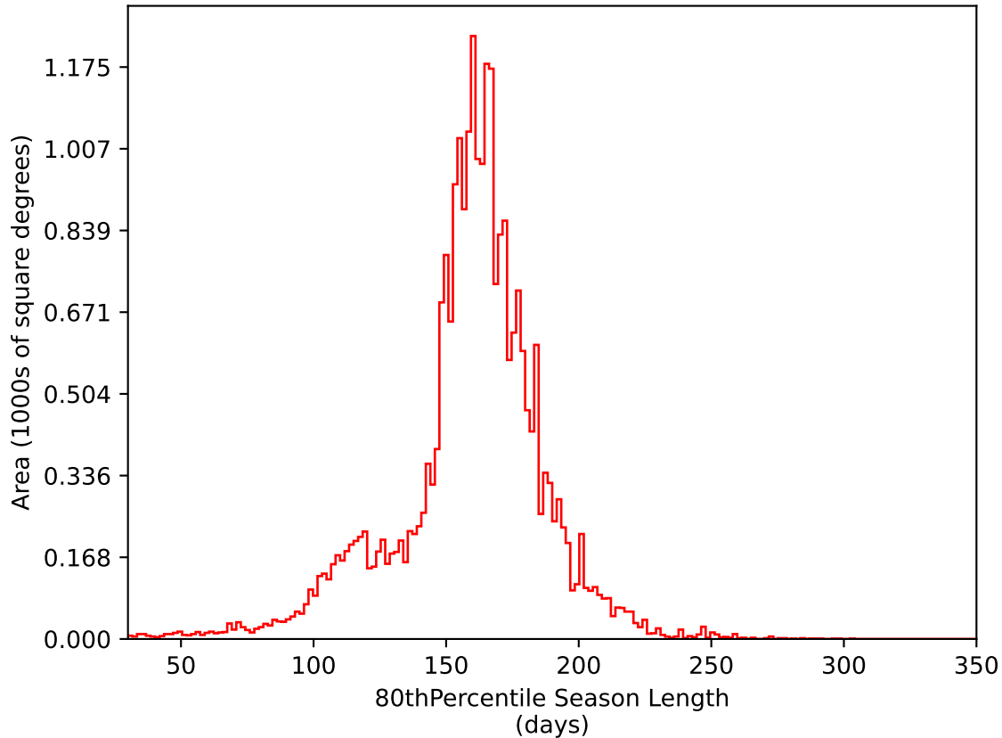
too_elab_r32_d2_ugrizy_v3.4_10yrs All sky i band: 80thPercentile Season Length
