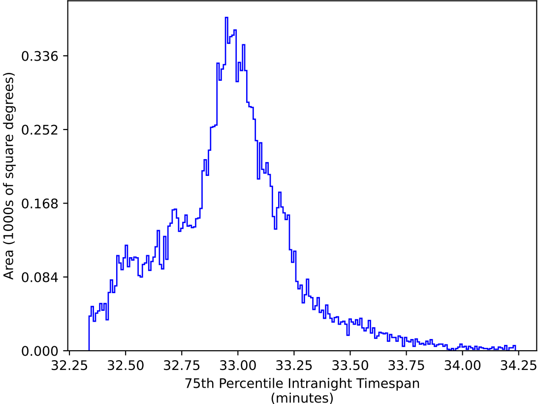
too_elab_r32_d2_ugrizy_v3.4_10yrs WFD y band: 75th Percentile Intranight Timespan
