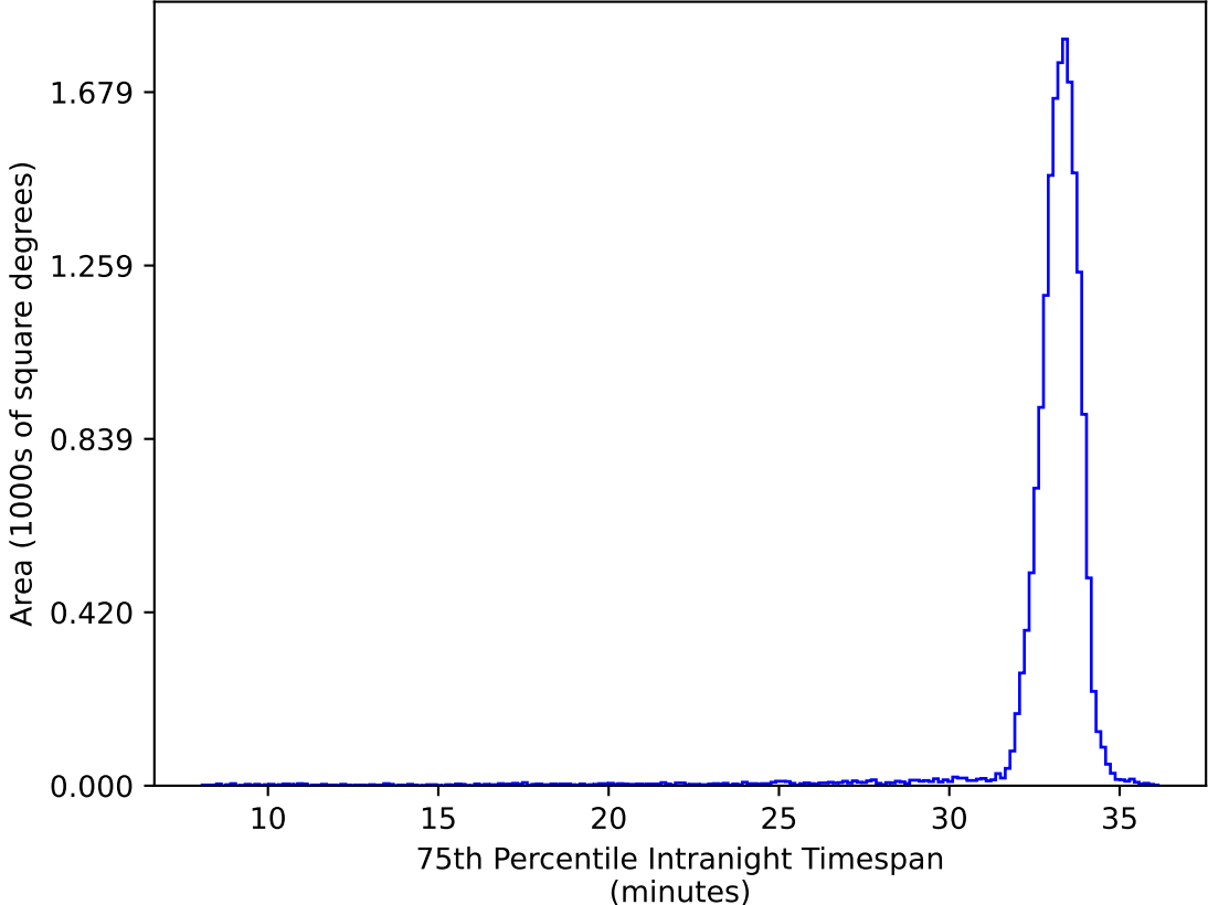
too_elab_r32_d2_ugrizy_v3.4_10yrs WFD ug bands: 75th Percentile Intranight Timespan
