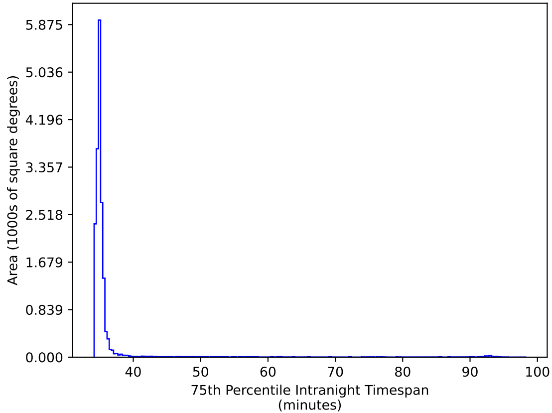
too_elab_r32_d2_ugrizy_v3.4_10yrs WFD ri bands: 75th Percentile Intranight Timespan
