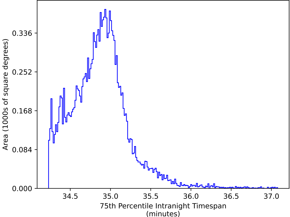
too_elab_r32_d2_ugrizy_v3.4_10yrs WFD iz bands: 75th Percentile Intranight Timespan
