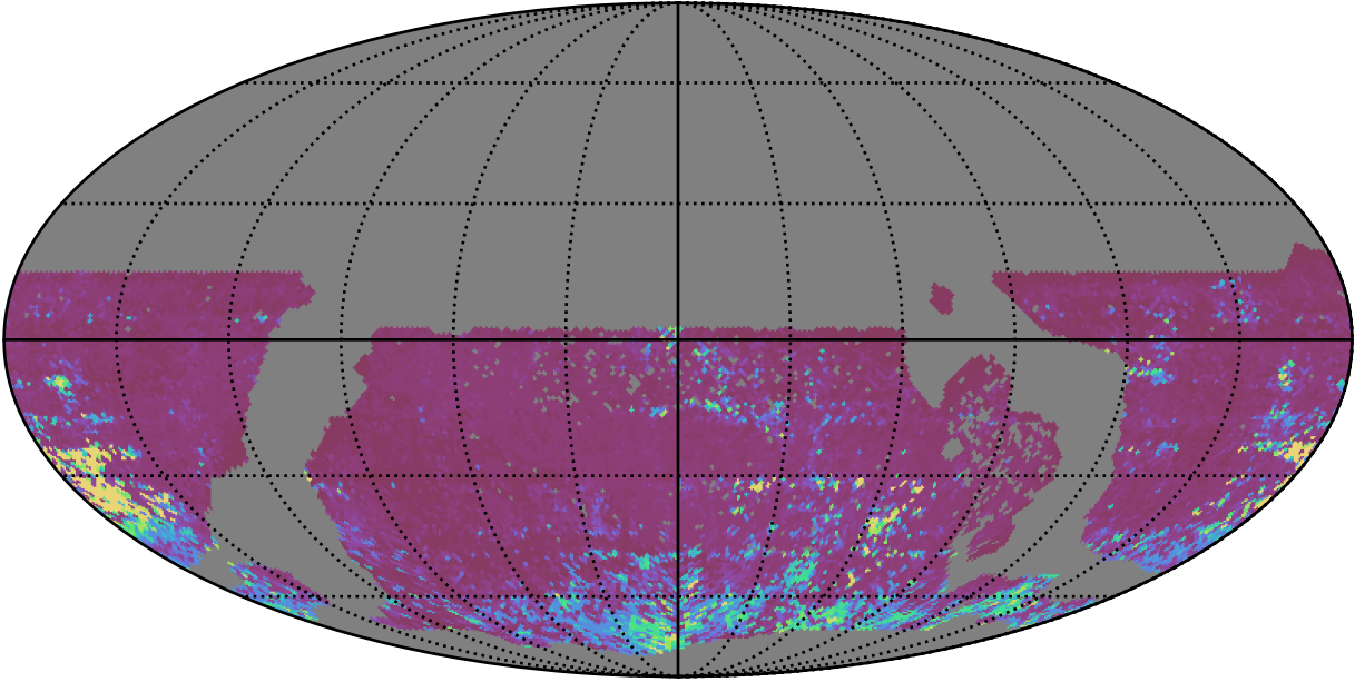
too_elab_r32_d2_ugrizy_v3.4_10yrs WFD i band: 75th Percentile Intranight Timespan
