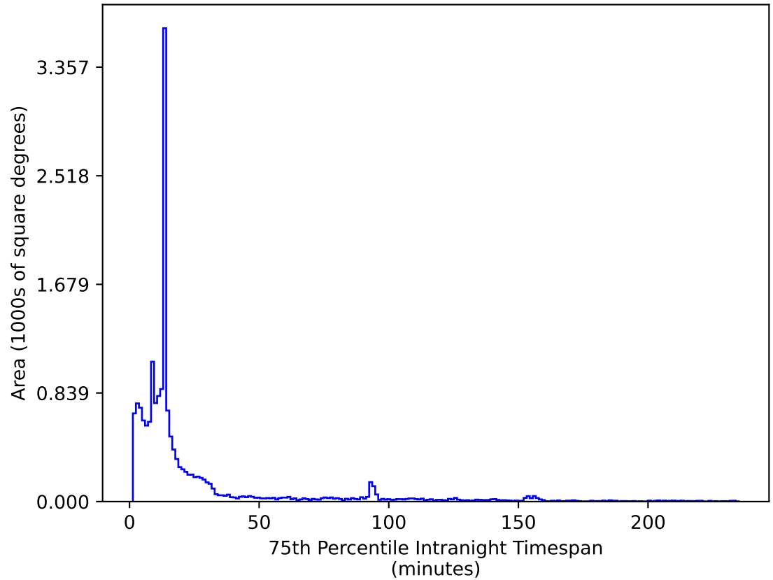
too_elab_r32_d2_ugrizy_v3.4_10yrs WFD i band: 75th Percentile Intranight Timespan
