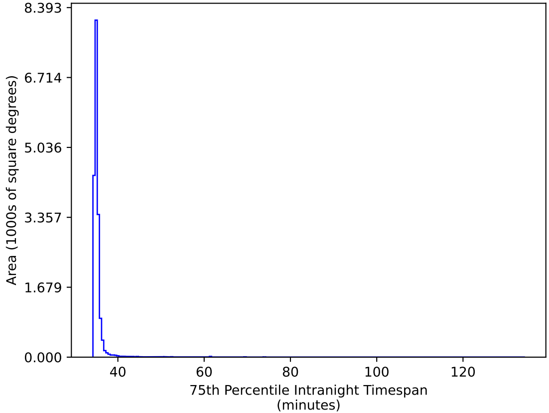
too_elab_r32_d2_ugrizy_v3.4_10yrs WFD gr bands: 75th Percentile Intranight Timespan
