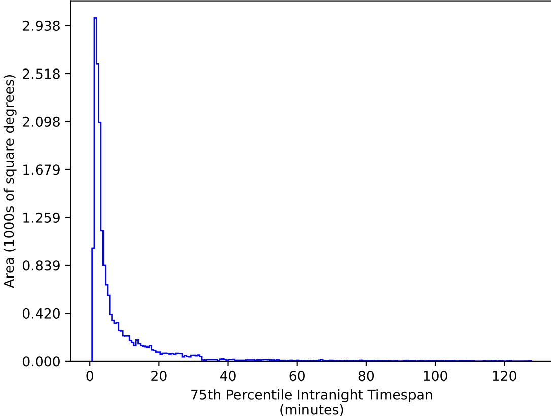
too_elab_r32_d2_ugrizy_v3.4_10yrs WFD g band: 75th Percentile Intranight Timespan
