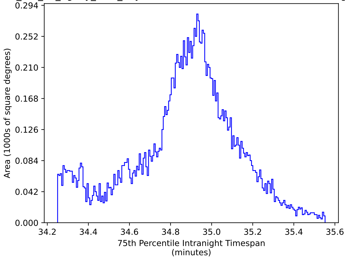
too_elab_r32_d2_ugrizy_v3.4_10yrs WFD all bands: 75th Percentile Intranight Timespan
