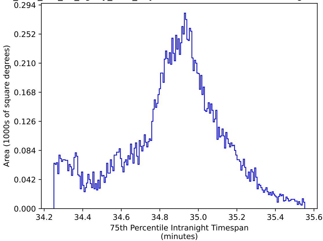
too_elab_r32_d2_ugrizy_v3.4_10yrs WFD: 75th Percentile Intranight Timespan
