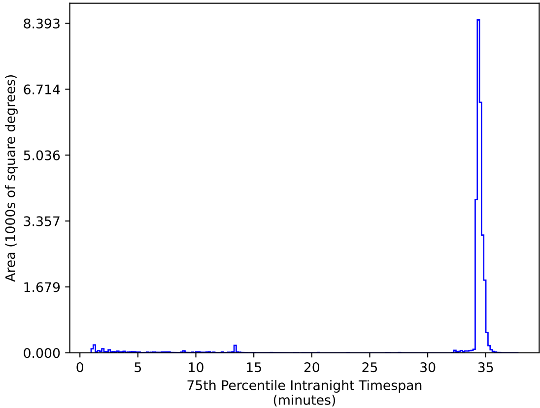
too_elab_r32_d2_ugrizy_v3.4_10yrs All sky zy bands: 75th Percentile Intranight Timespan
