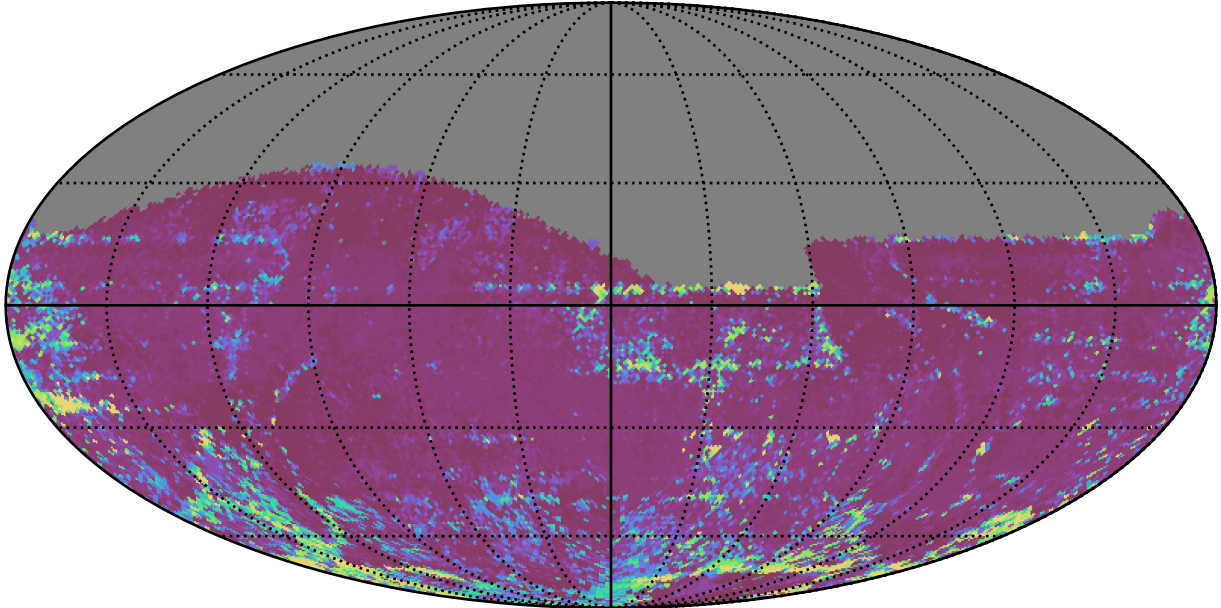
too_elab_r32_d2_ugrizy_v3.4_10yrs All sky z band: 75th Percentile Intranight Timespan
