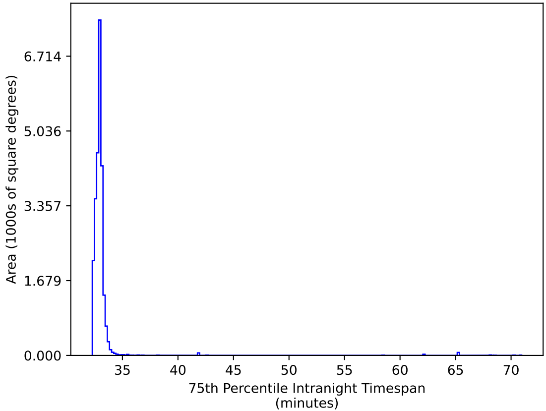
too_elab_r32_d2_ugrizy_v3.4_10yrs All sky y band: 75th Percentile Intranight Timespan
