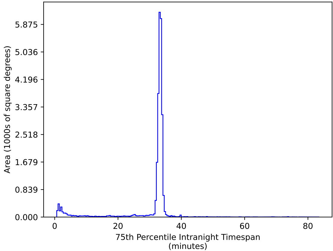
too_elab_r32_d2_ugrizy_v3.4_10yrs All sky ug bands: 75th Percentile Intranight Timespan
