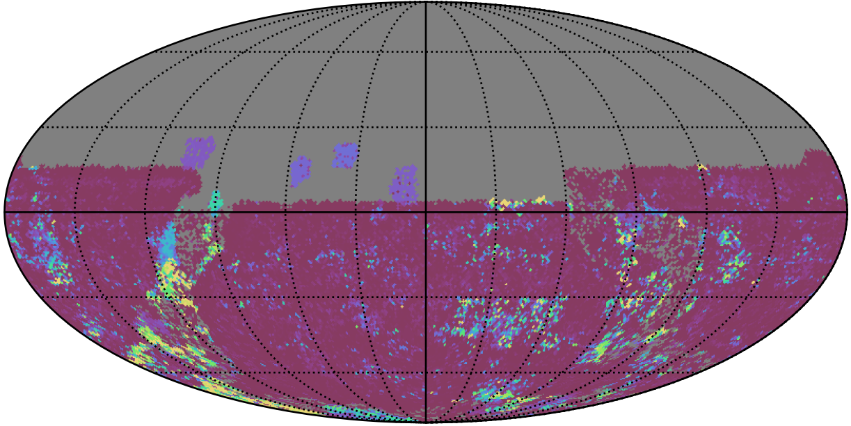
too_elab_r32_d2_ugrizy_v3.4_10yrs All sky u band: 75th Percentile Intranight Timespan
