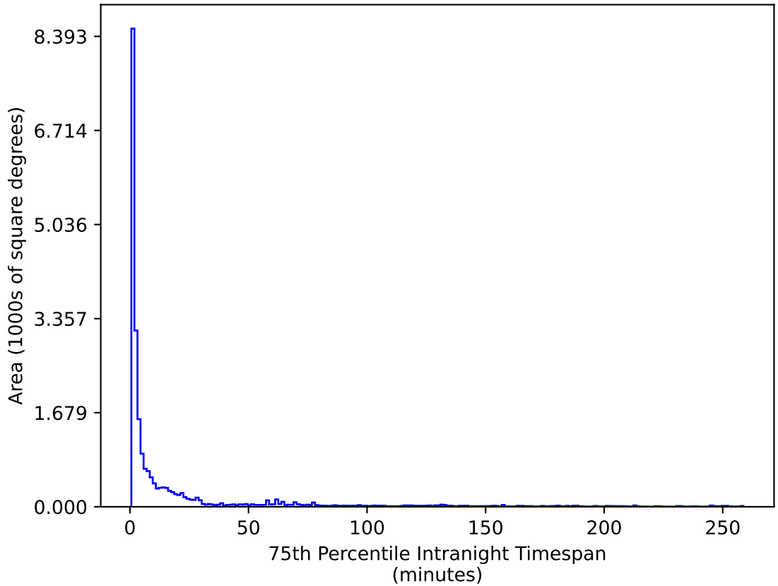
too_elab_r32_d2_ugrizy_v3.4_10yrs All sky u band: 75th Percentile Intranight Timespan
