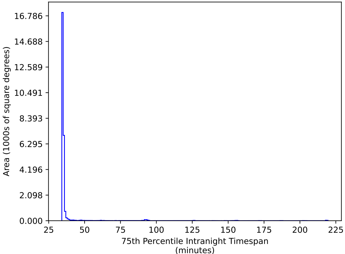
too_elab_r32_d2_ugrizy_v3.4_10yrs All sky ri bands: 75th Percentile Intranight Timespan
