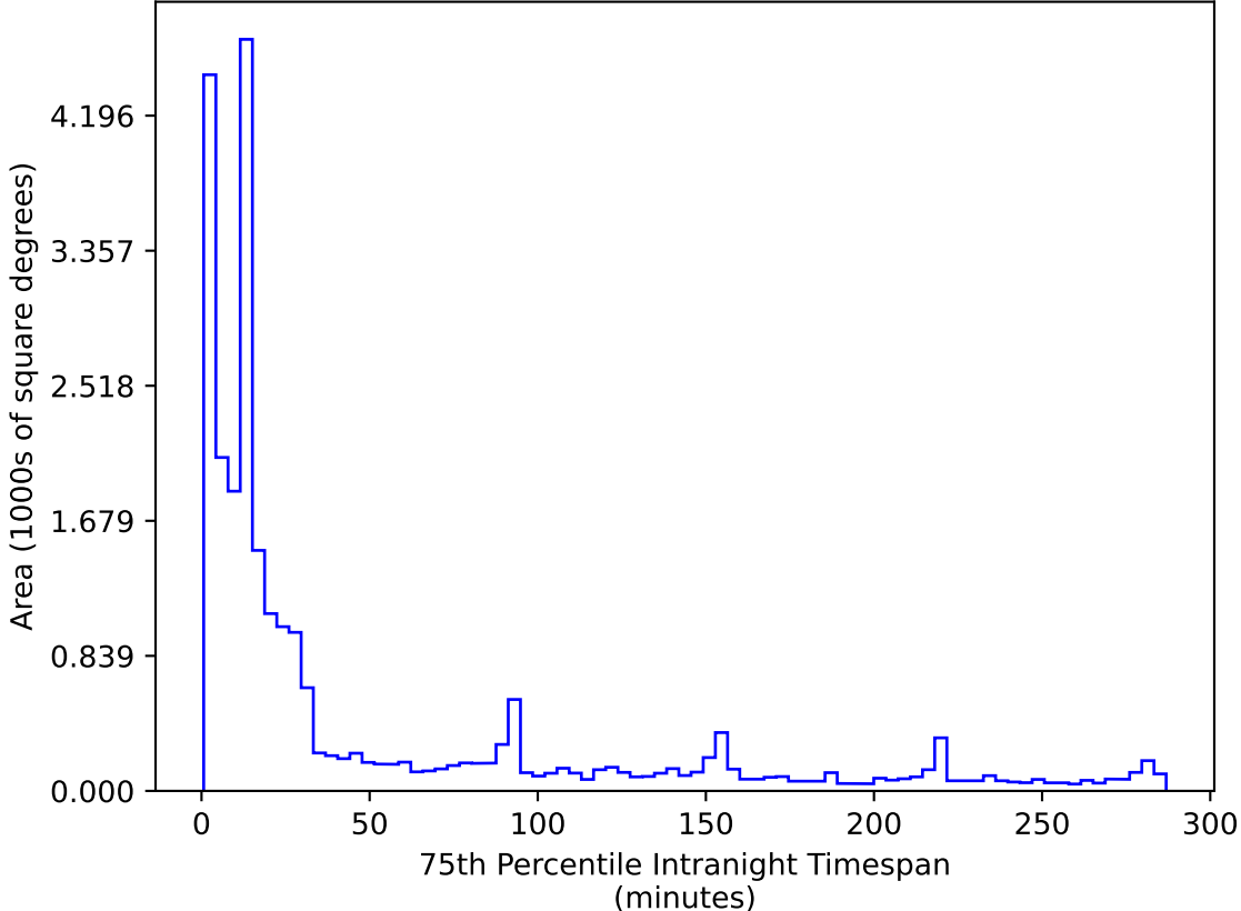
too_elab_r32_d2_ugrizy_v3.4_10yrs All sky r band: 75th Percentile Intranight Timespan
