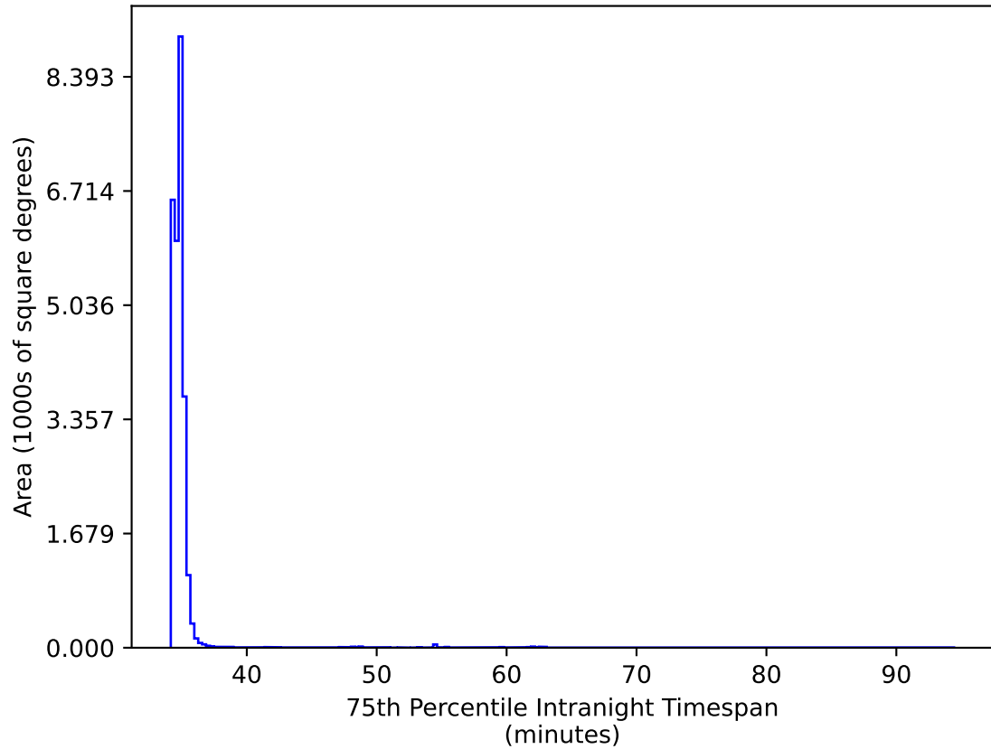
too_elab_r32_d2_ugrizy_v3.4_10yrs All sky iz bands: 75th Percentile Intranight Timespan
