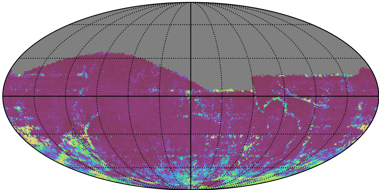
too_elab_r32_d2_ugrizy_v3.4_10yrs All sky i band: 75th Percentile Intranight Timespan
