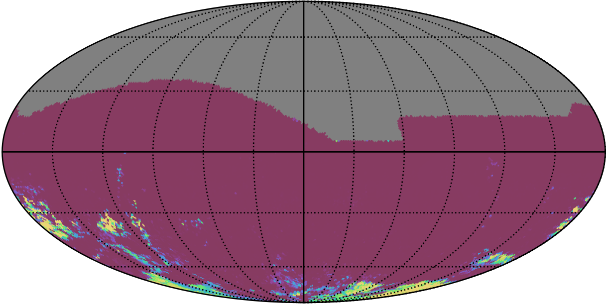
too_elab_r32_d2_ugrizy_v3.4_10yrs All sky gr bands: 75th Percentile Intranight Timespan
