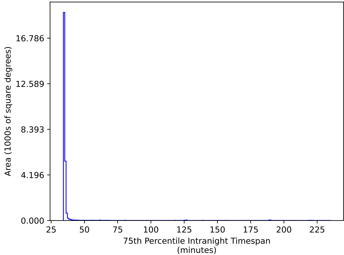
too_elab_r32_d2_ugrizy_v3.4_10yrs All sky gr bands: 75th Percentile Intranight Timespan
